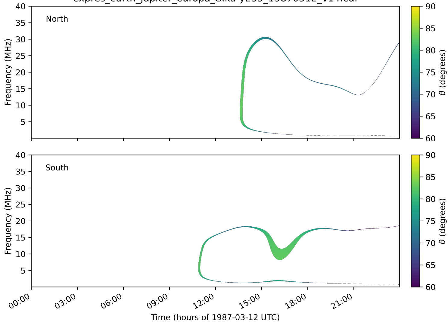
expres_earth_jupiter_europa_txka-y235_19870312_v14.cdf
