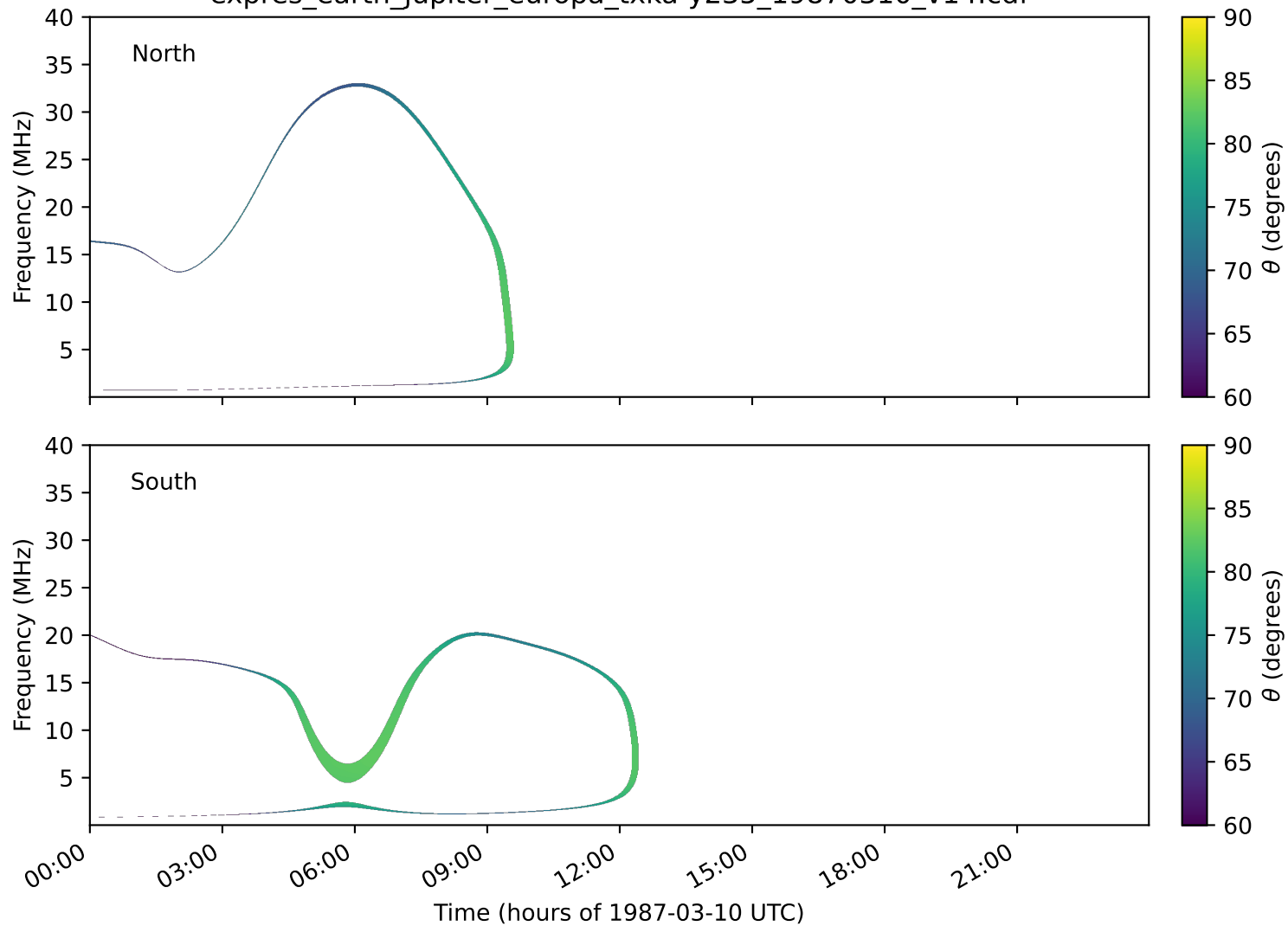
expres_earth_jupiter_europa_txka-y235_19870310_v14.cdf
