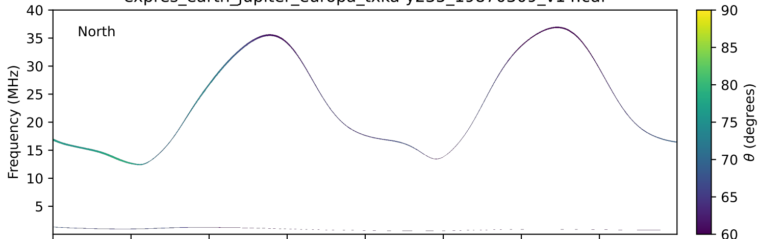
expres_earth_jupiter_europa_txka-y235_19870309_v14.cdf
