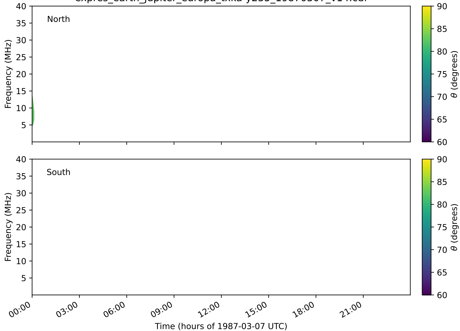
expres_earth_jupiter_europa_txka-y235_19870307_v14.cdf
