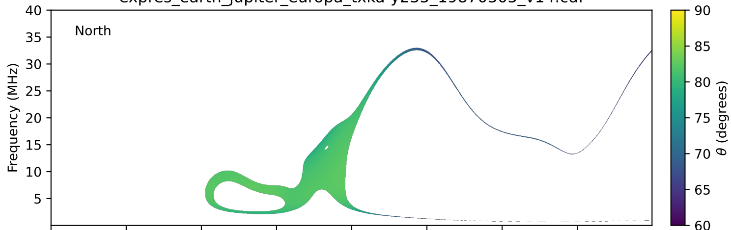
expres_earth_jupiter_europa_txka-y235_19870305_v14.cdf
