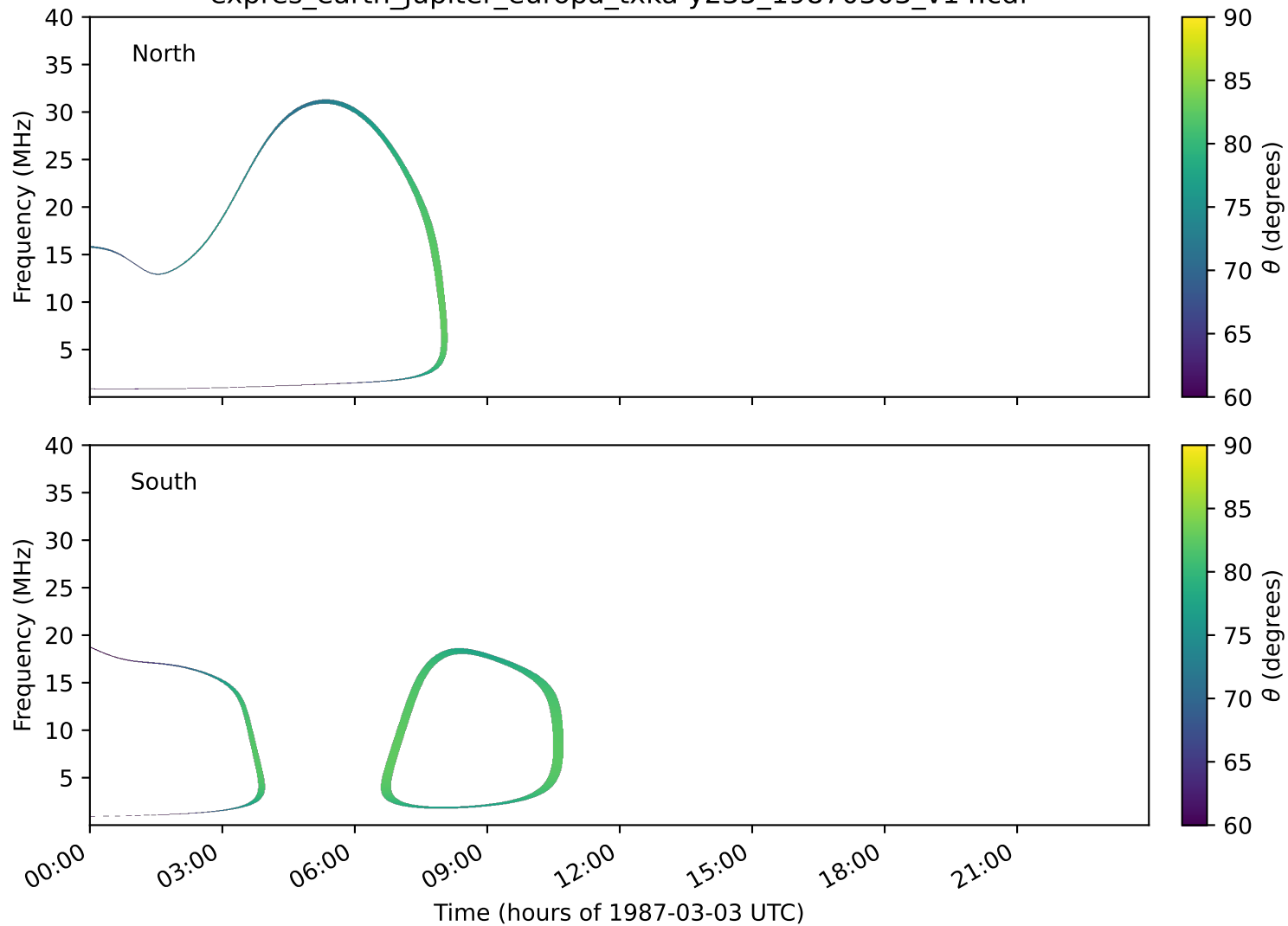
expres_earth_jupiter_europa_txka-y235_19870303_v14.cdf
