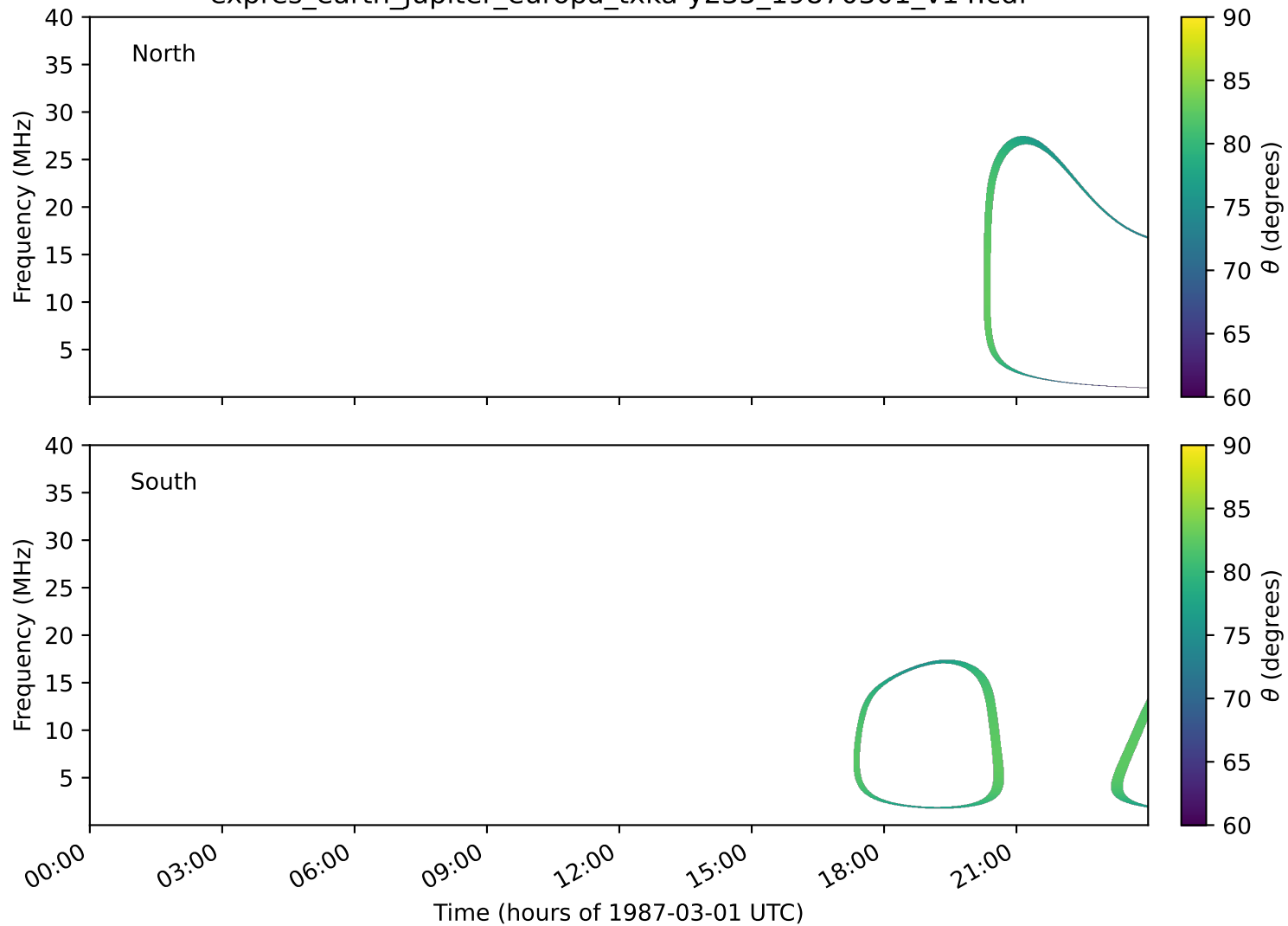
expres_earth_jupiter_europa_txka-y235_19870301_v14.cdf
