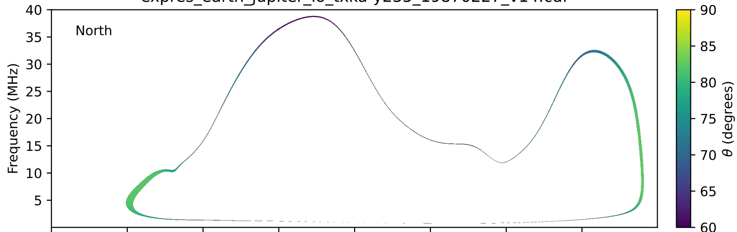
expres_earth_jupiter_io_txka-y235_19870227_v14.cdf
