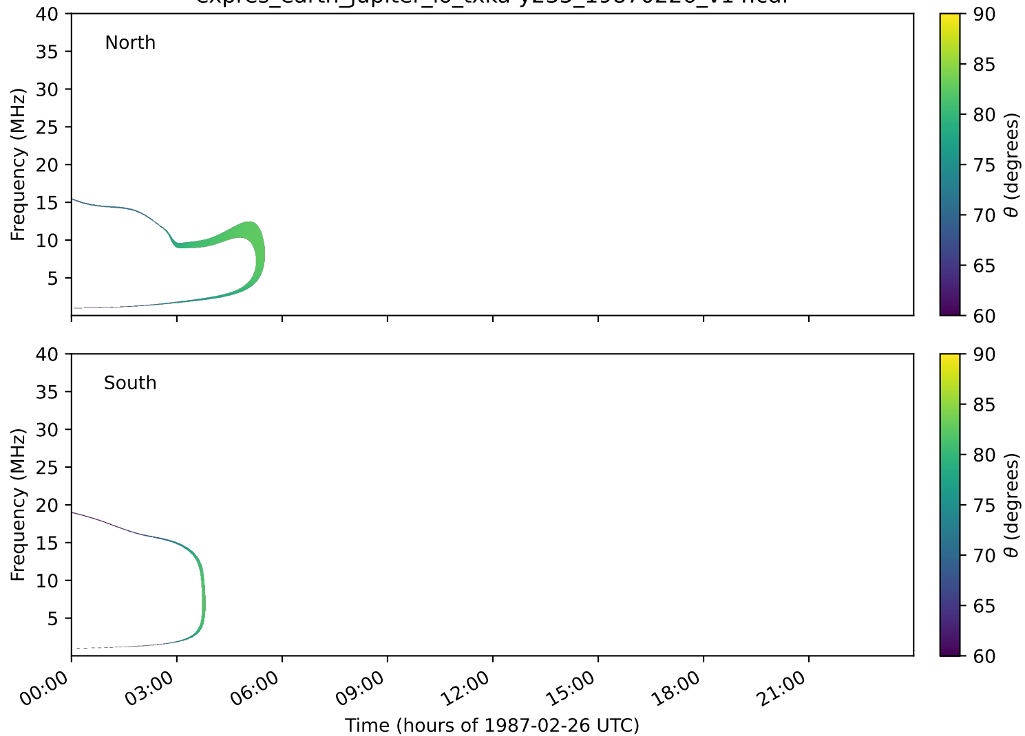
expres_earth_jupiter_io_txka-y235_19870226_v14.cdf
