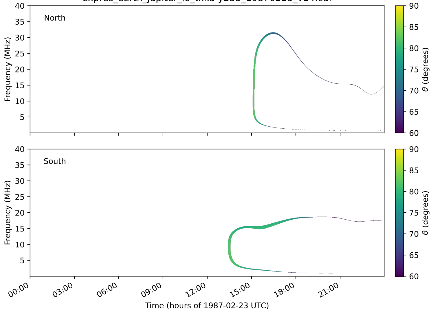
expres_earth_jupiter_io_txka-y235_19870223_v14.cdf
