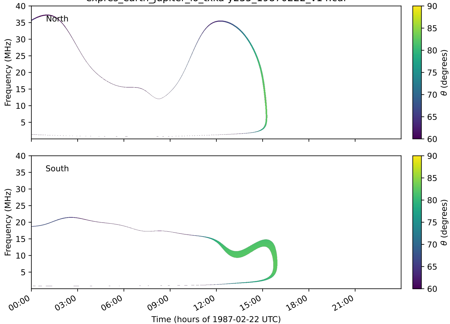
expres_earth_jupiter_io_txka-y235_19870222_v14.cdf
