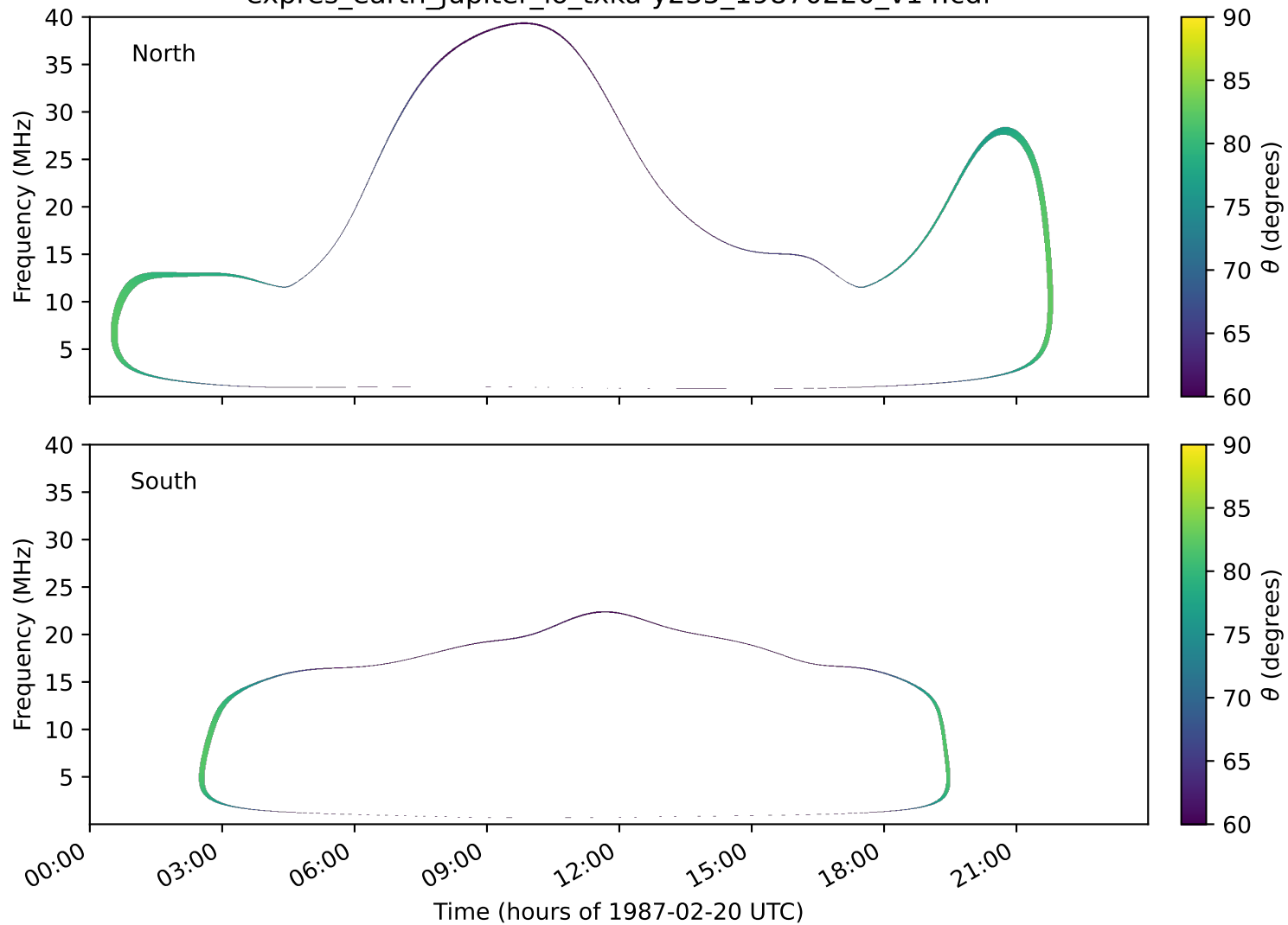
expres_earth_jupiter_io_txka-y235_19870220_v14.cdf
