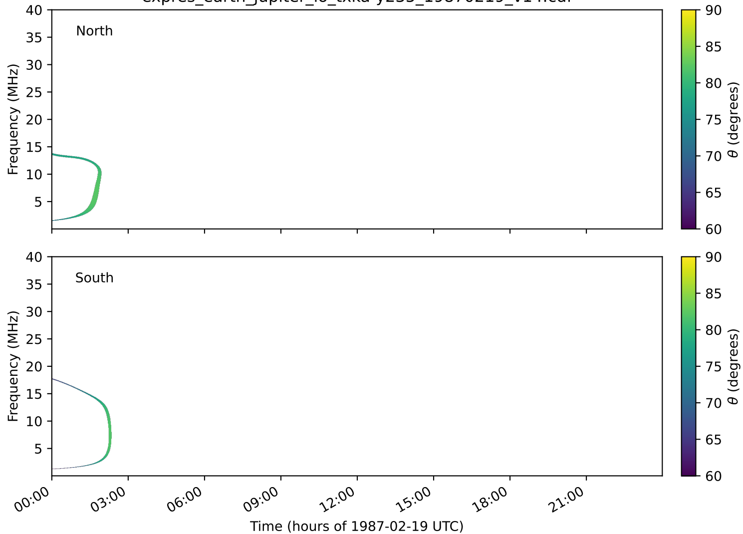
expres_earth_jupiter_io_txka-y235_19870219_v14.cdf
