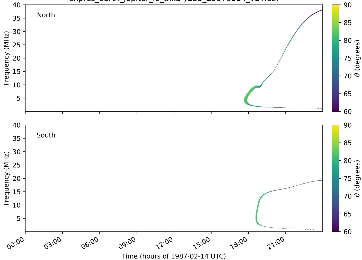
expres_earth_jupiter_io_txka-y235_19870214_v14.cdf
