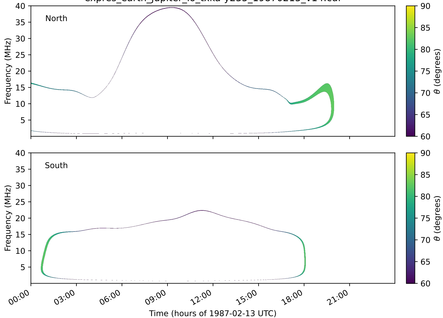
expres_earth_jupiter_io_txka-y235_19870213_v14.cdf
