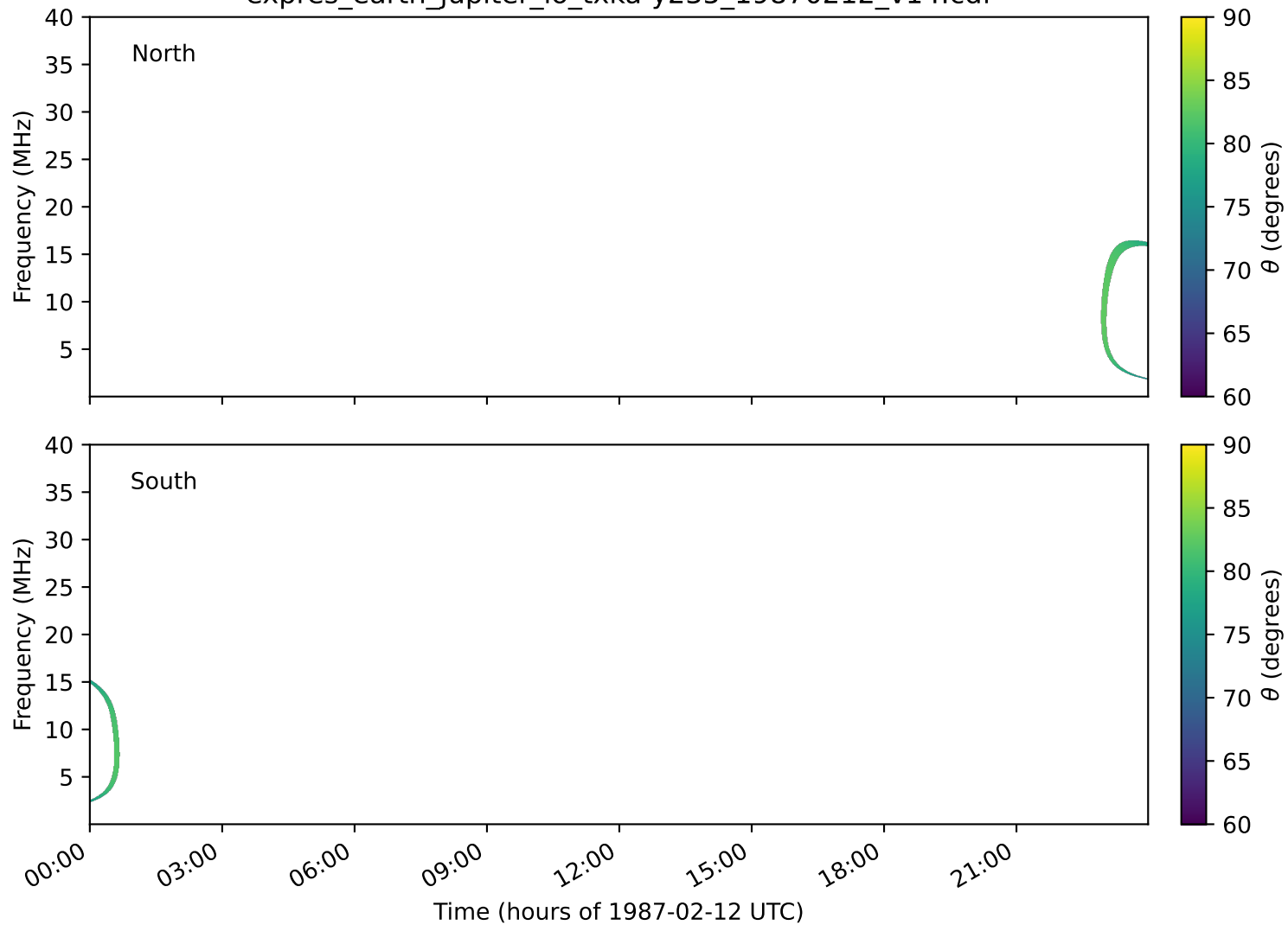
expres_earth_jupiter_io_txka-y235_19870212_v14.cdf
