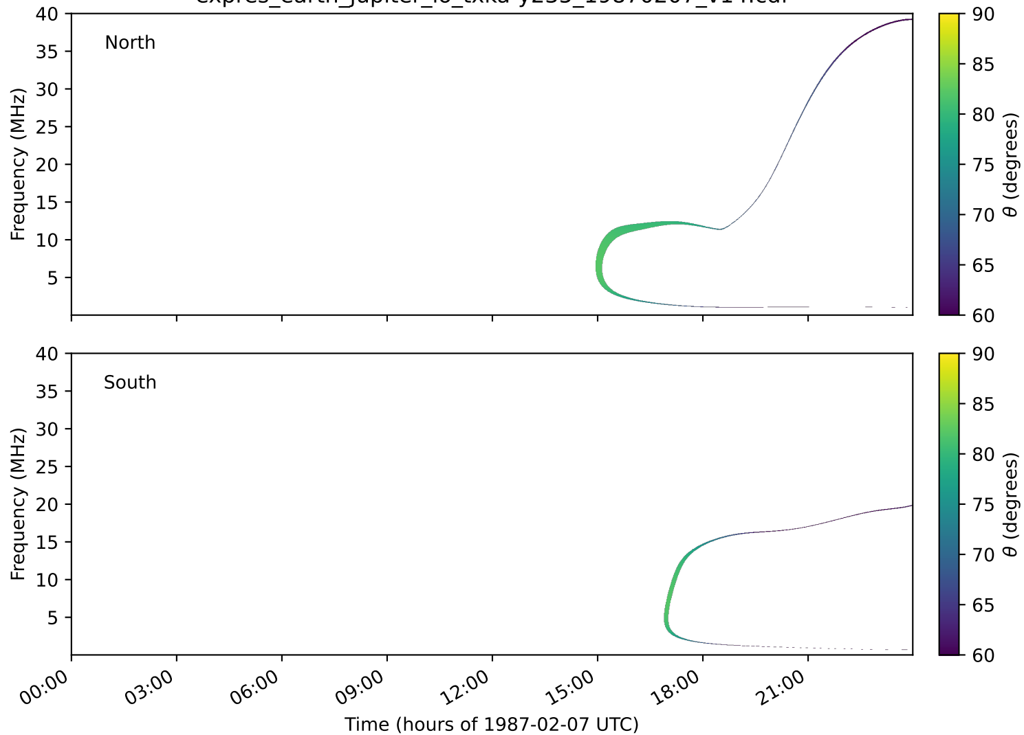
expres_earth_jupiter_io_txka-y235_19870207_v14.cdf
