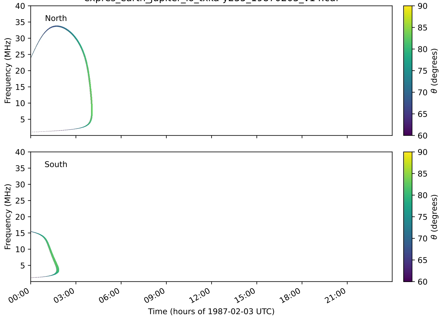
expres_earth_jupiter_io_txka-y235_19870203_v14.cdf
