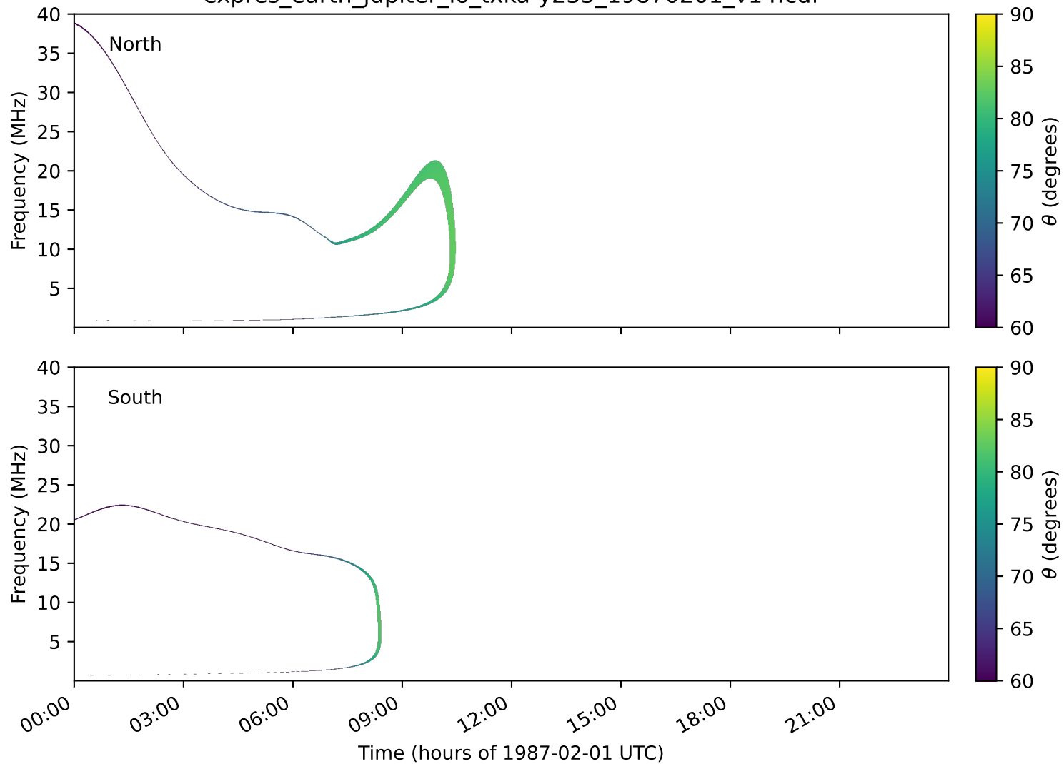
expres_earth_jupiter_io_txka-y235_19870201_v14.cdf
