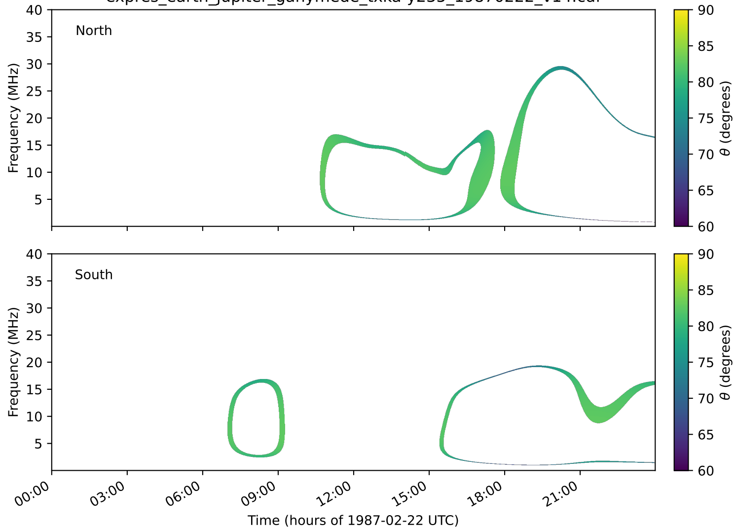
expres_earth_jupiter_ganymede_txka-y235_19870222_v14.cdf
