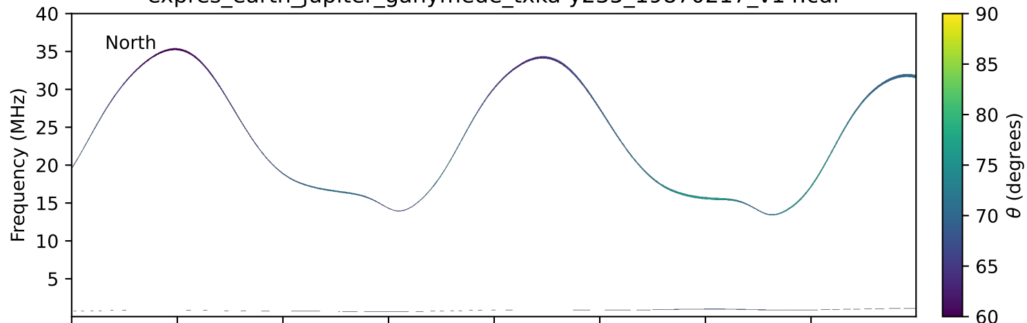
expres_earth_jupiter_ganymede_txka-y235_19870217_v14.cdf
