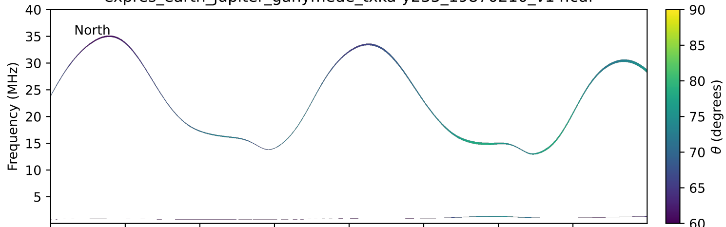
expres_earth_jupiter_ganymede_txka-y235_19870210_v14.cdf
