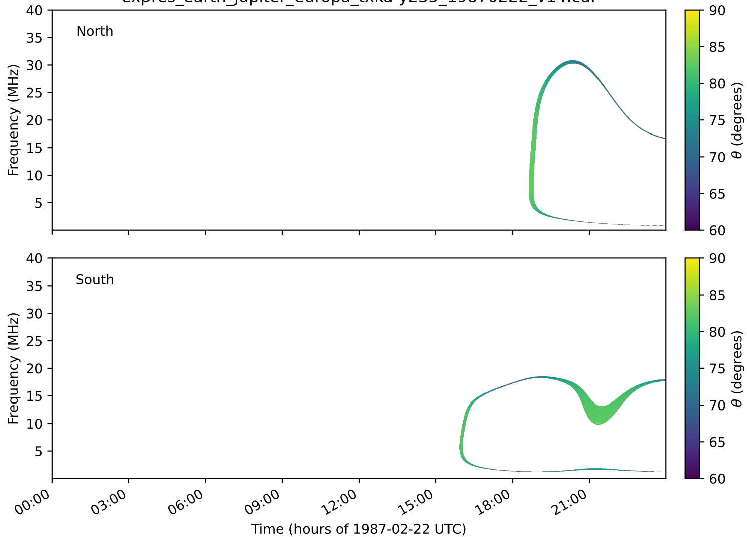
expres_earth_jupiter_europa_txka-y235_19870222_v14.cdf
