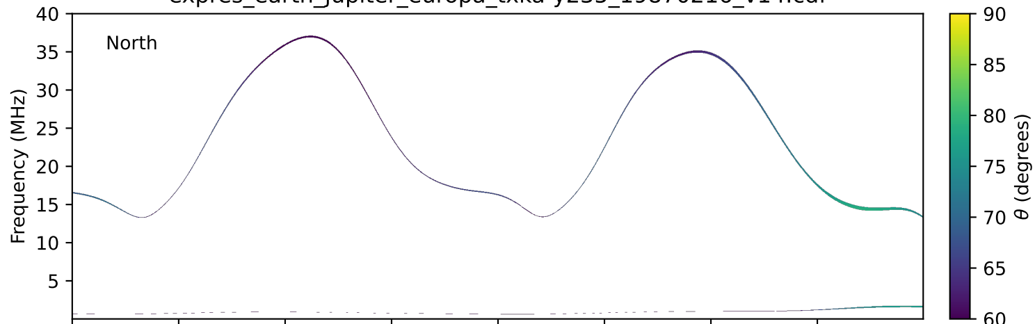
expres_earth_jupiter_europa_txka-y235_19870216_v14.cdf
