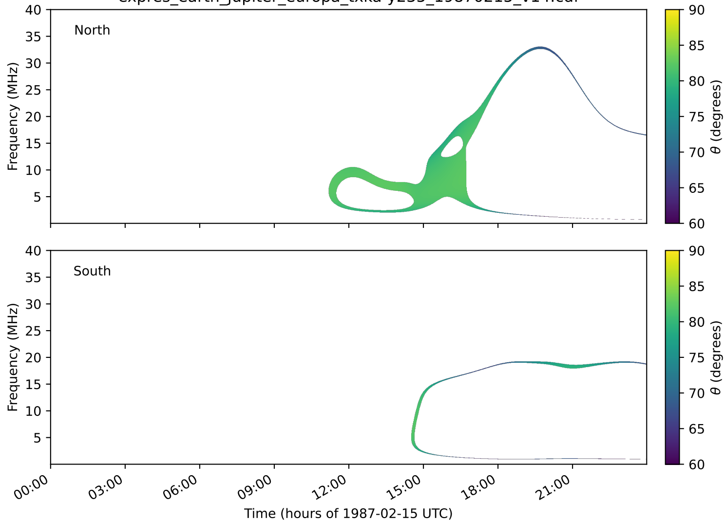
expres_earth_jupiter_europa_txka-y235_19870215_v14.cdf
