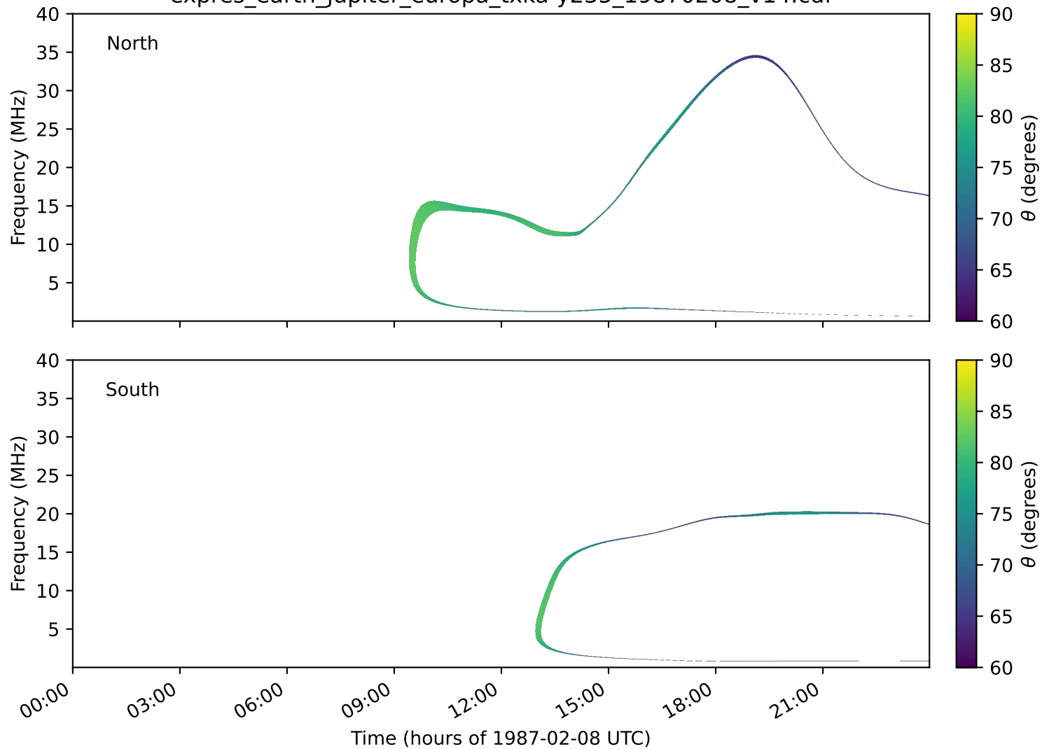
expres_earth_jupiter_europa_txka-y235_19870208_v14.cdf
