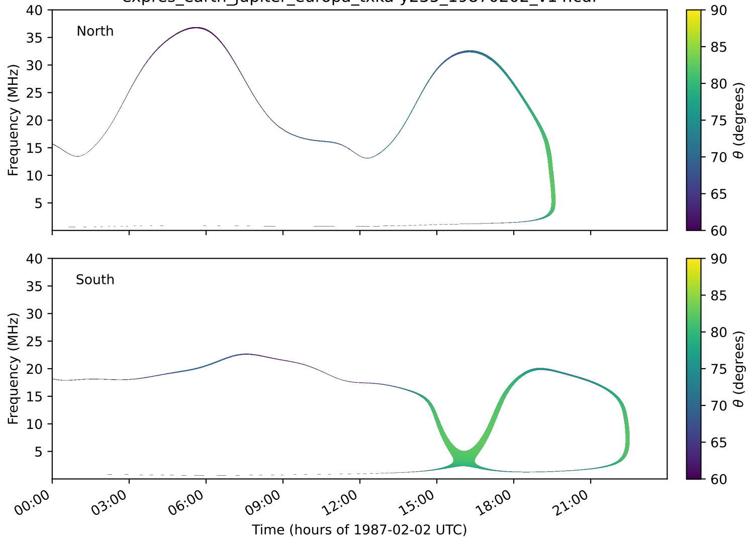
expres_earth_jupiter_europa_txka-y235_19870202_v14.cdf
