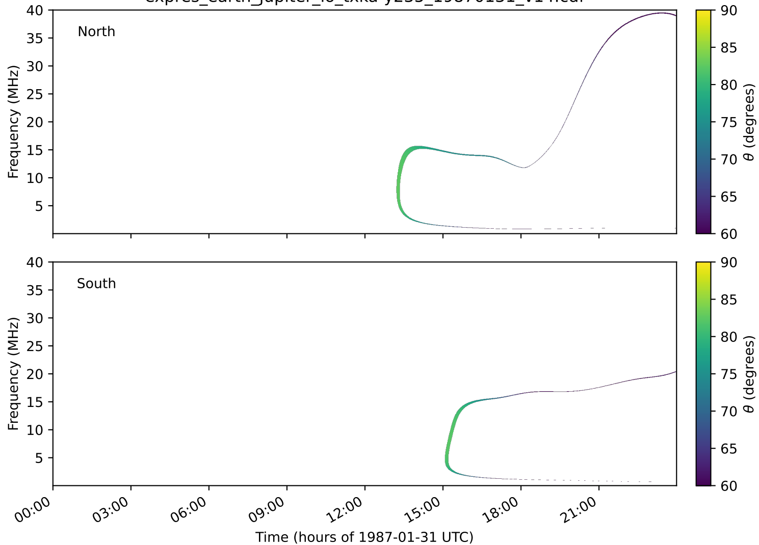
expres_earth_jupiter_io_txka-y235_19870131_v14.cdf
