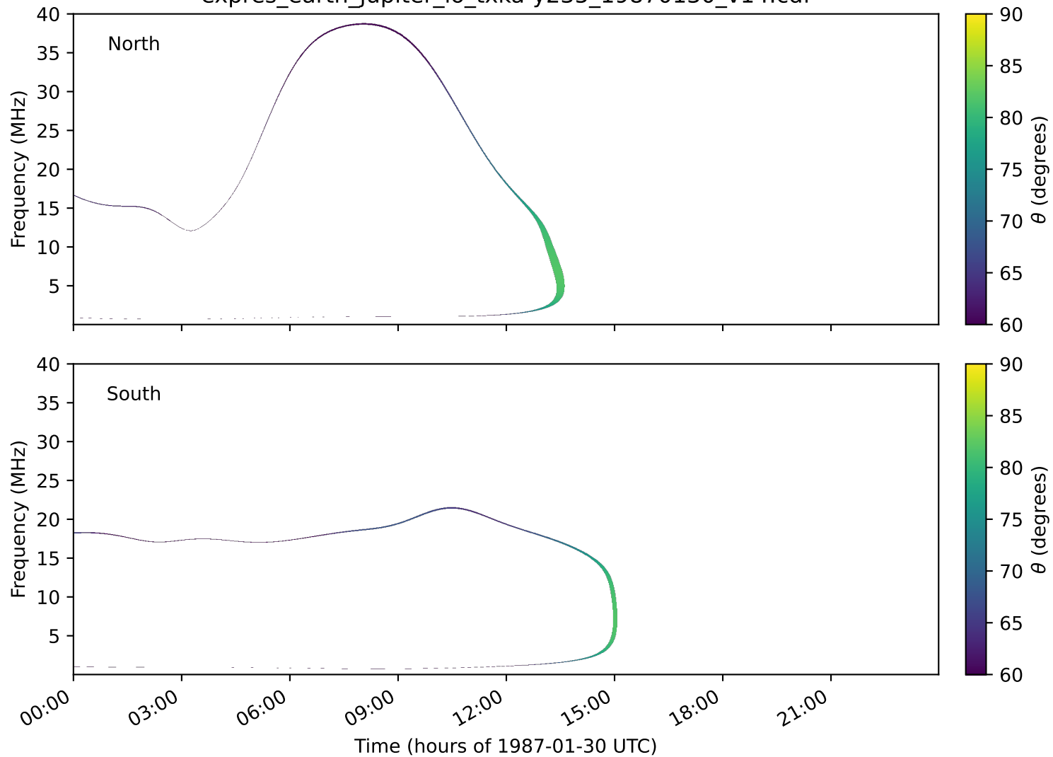
expres_earth_jupiter_io_txka-y235_19870130_v14.cdf
