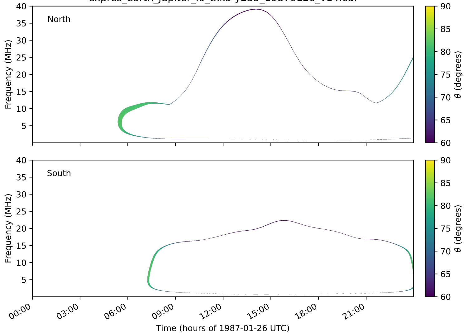
expres_earth_jupiter_io_txka-y235_19870126_v14.cdf
