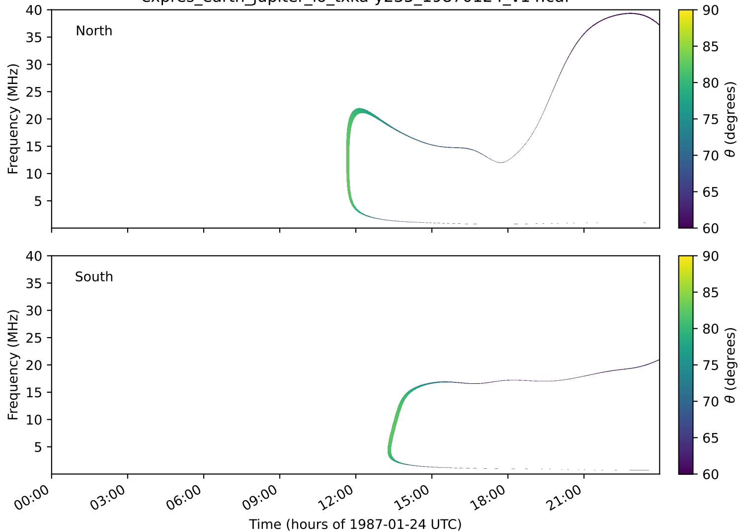
expres_earth_jupiter_io_txka-y235_19870124_v14.cdf
