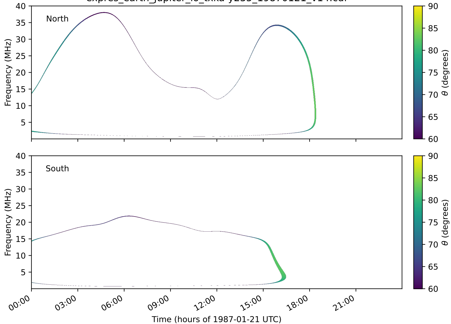
expres_earth_jupiter_io_txka-y235_19870121_v14.cdf
