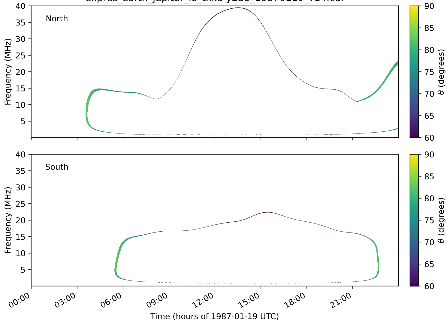
expres_earth_jupiter_io_txka-y235_19870119_v14.cdf
