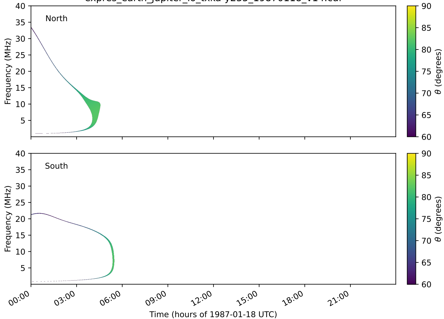
expres_earth_jupiter_io_txka-y235_19870118_v14.cdf
