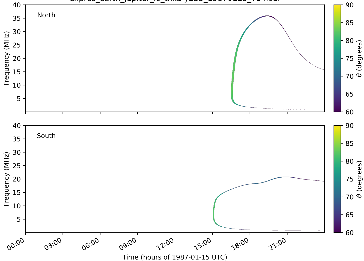
expres_earth_jupiter_io_txka-y235_19870115_v14.cdf
