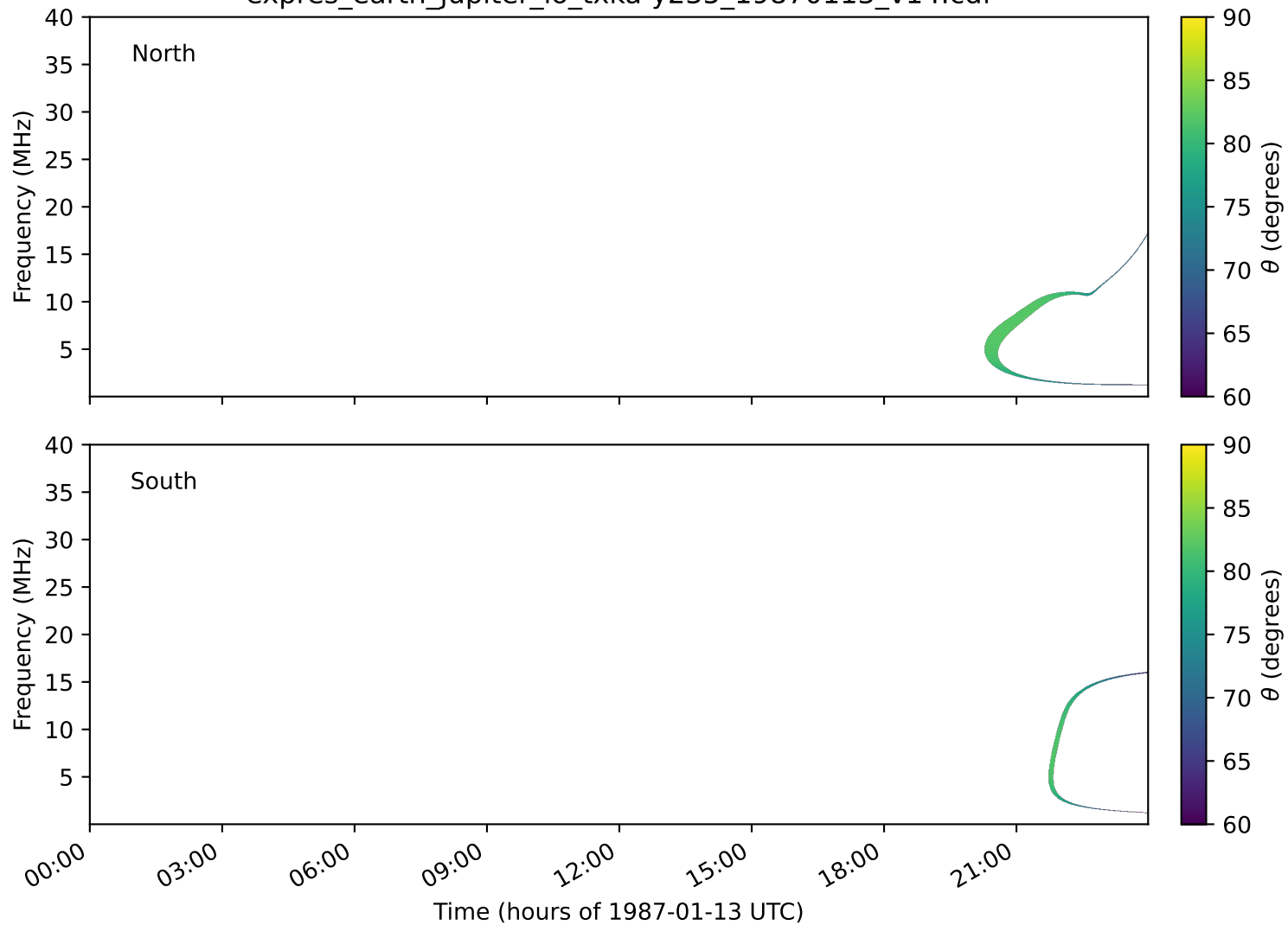
expres_earth_jupiter_io_txka-y235_19870113_v14.cdf
