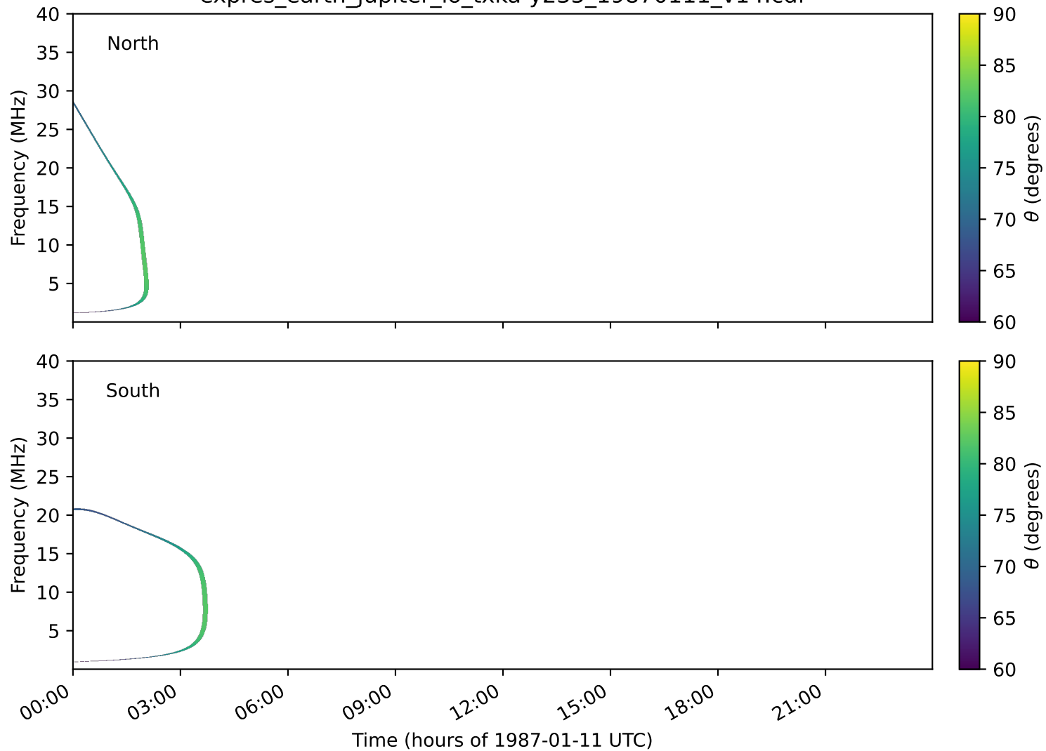
expres_earth_jupiter_io_txka-y235_19870111_v14.cdf
