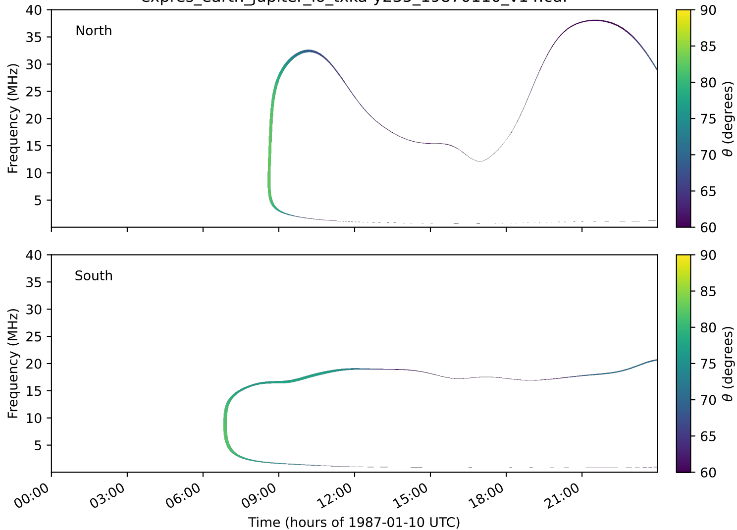
expres_earth_jupiter_io_txka-y235_19870110_v14.cdf
