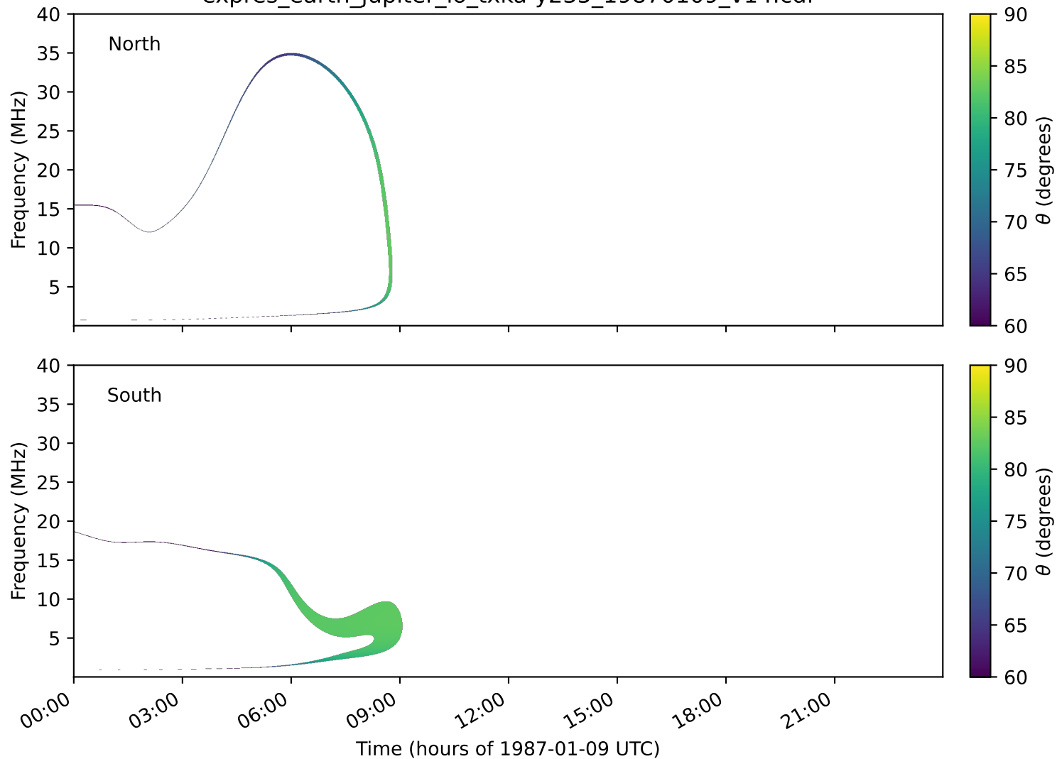
expres_earth_jupiter_io_txka-y235_19870109_v14.cdf
