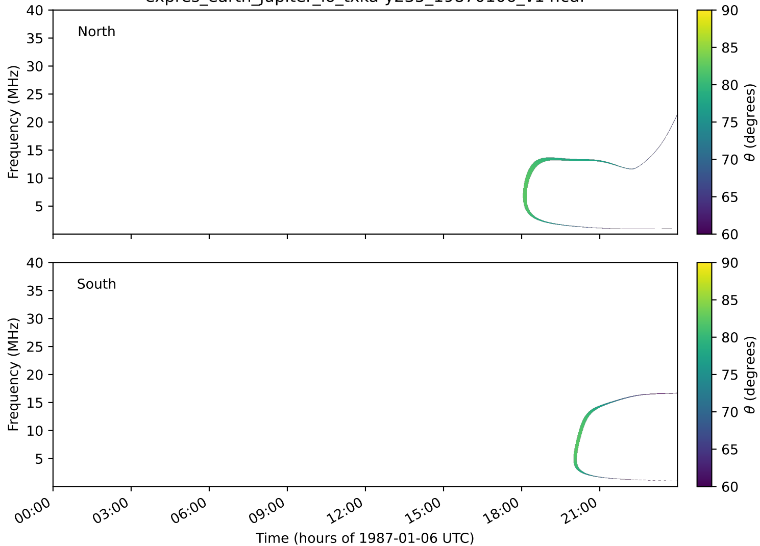
expres_earth_jupiter_io_txka-y235_19870106_v14.cdf
