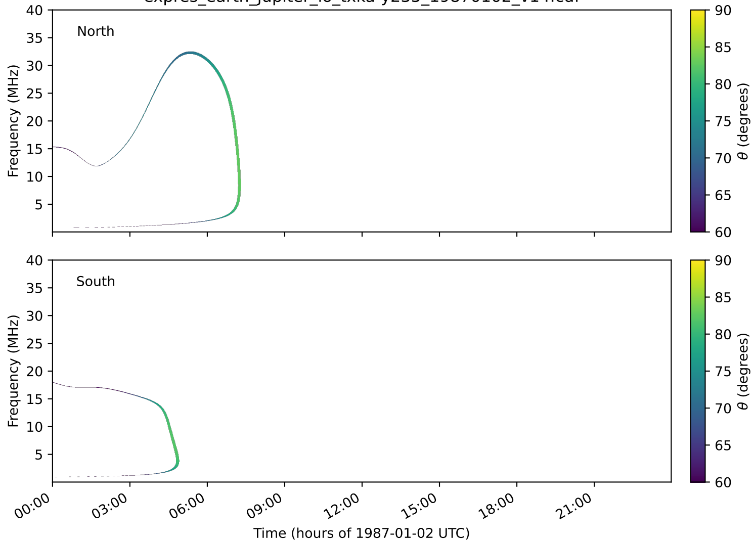
expres_earth_jupiter_io_txka-y235_19870102_v14.cdf
