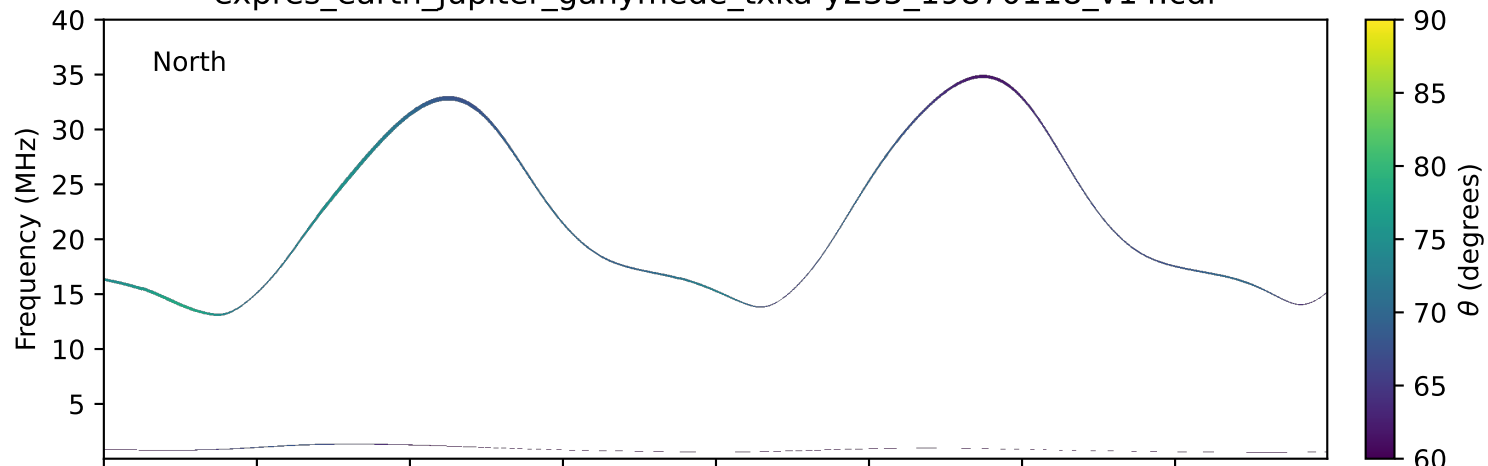
expres_earth_jupiter_ganymede_txka-y235_19870118_v14.cdf
