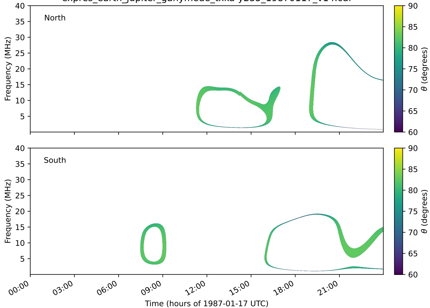
expres_earth_jupiter_ganymede_txka-y235_19870117_v14.cdf
