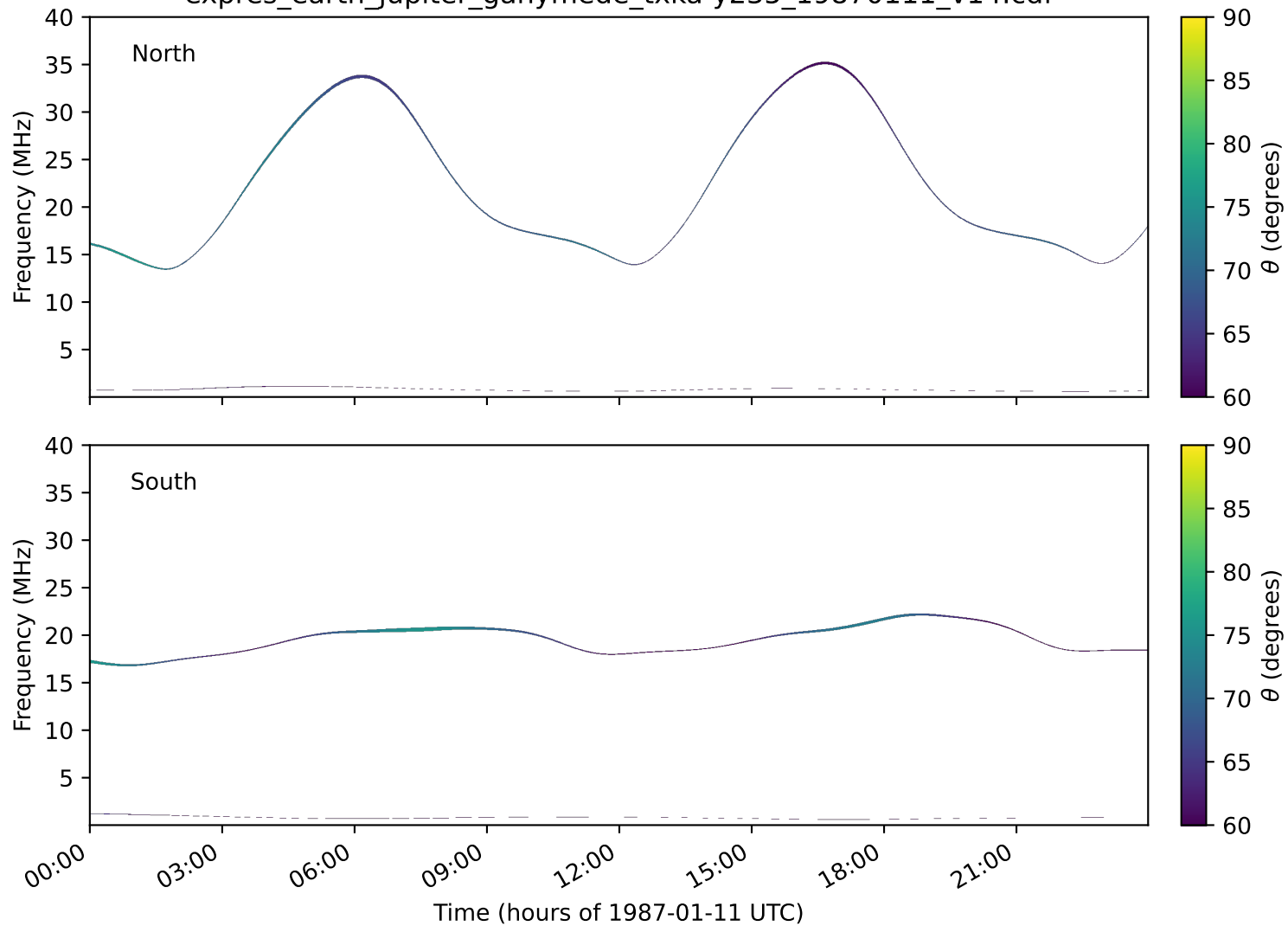
expres_earth_jupiter_ganymede_txka-y235_19870111_v14.cdf
