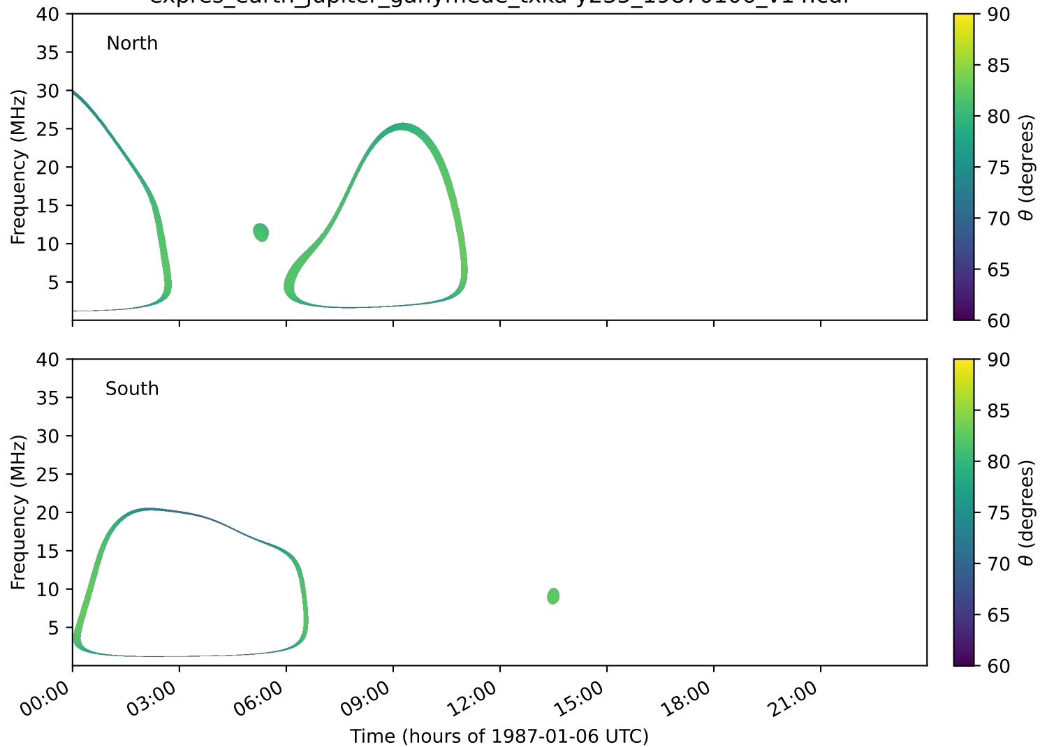
expres_earth_jupiter_ganymede_txka-y235_19870106_v14.cdf
