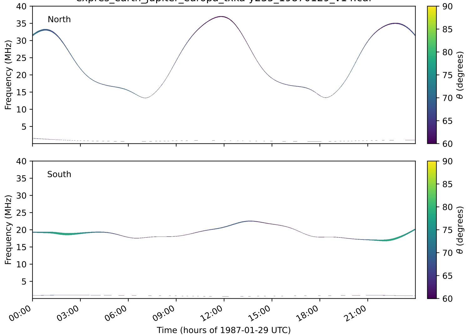
expres_earth_jupiter_europa_txka-y235_19870129_v14.cdf
