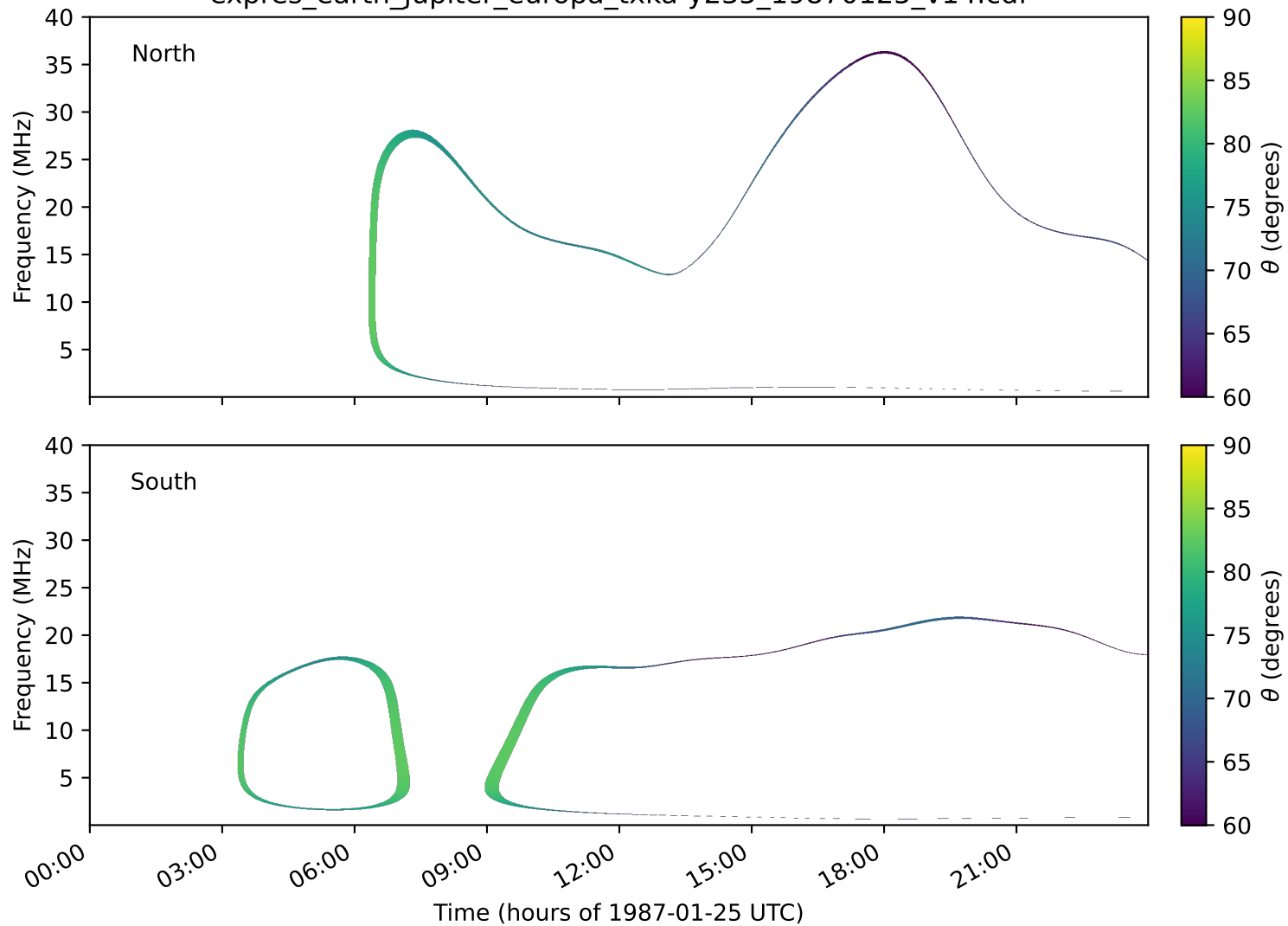
expres_earth_jupiter_europa_txka-y235_19870125_v14.cdf
