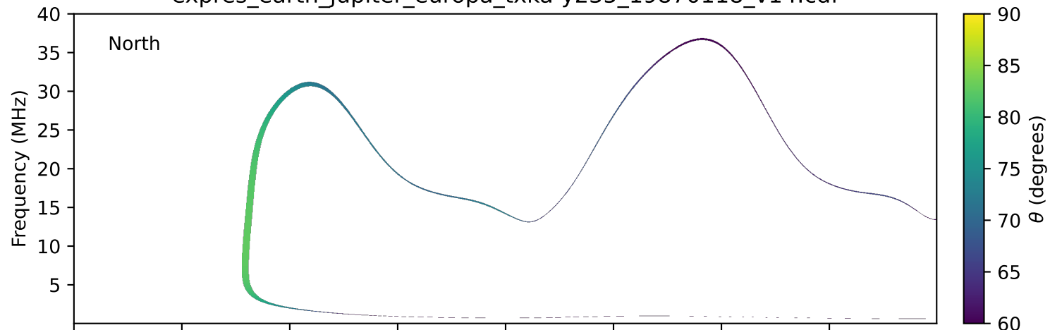
expres_earth_jupiter_europa_txka-y235_19870118_v14.cdf
