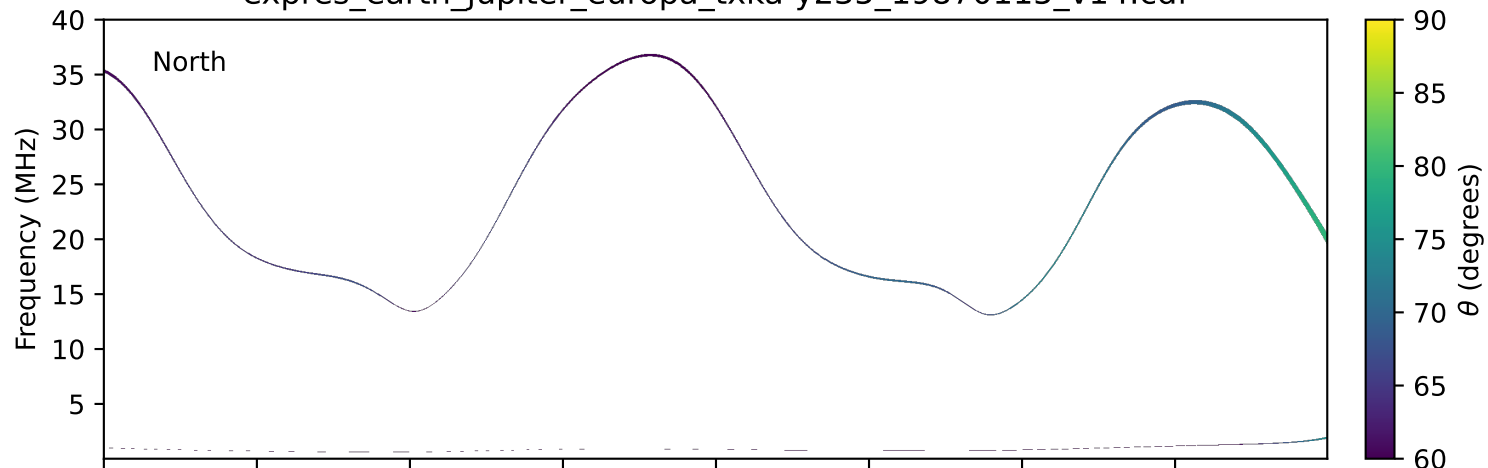
expres_earth_jupiter_europa_txka-y235_19870115_v14.cdf
