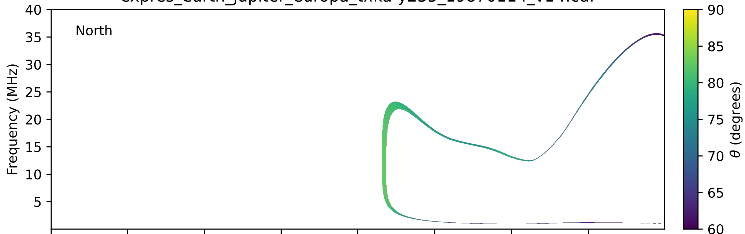
expres_earth_jupiter_europa_txka-y235_19870114_v14.cdf
